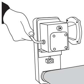
1 Remove lowest plug from speed reducer.
